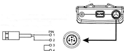
Connection for 2-wire electret condenser microphone
