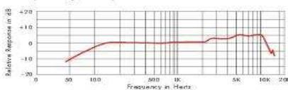
Frequency Graph :
